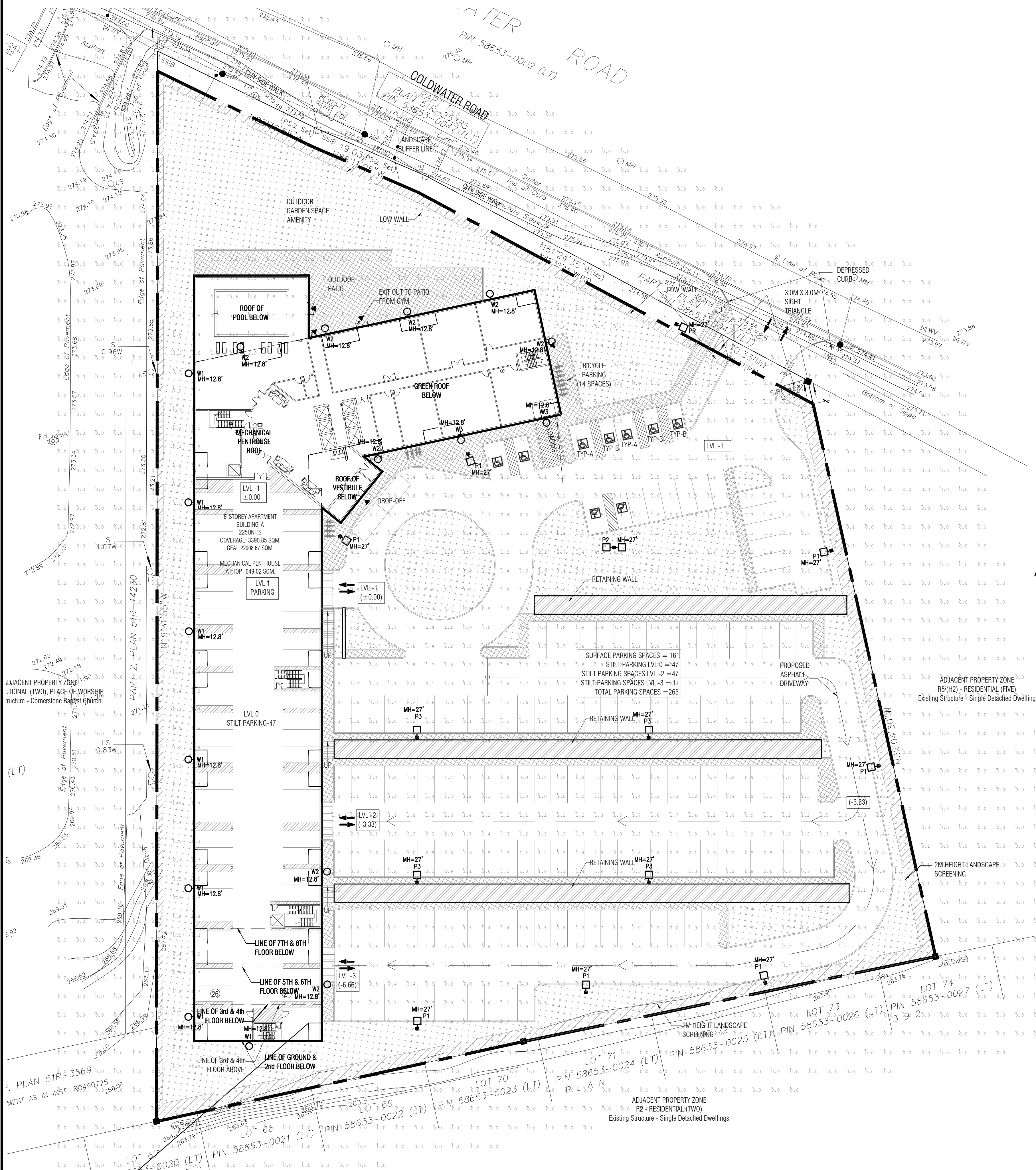
1 SITE PLAN - ELECTRICAL LAYOUT E-1.1 1:350
